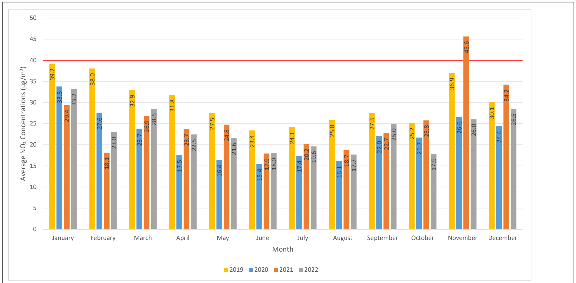
Figure A.8 – Trends in Monthly Average NO 2 Concentrations from Twyford Continuous Monitor for 2019-2022
