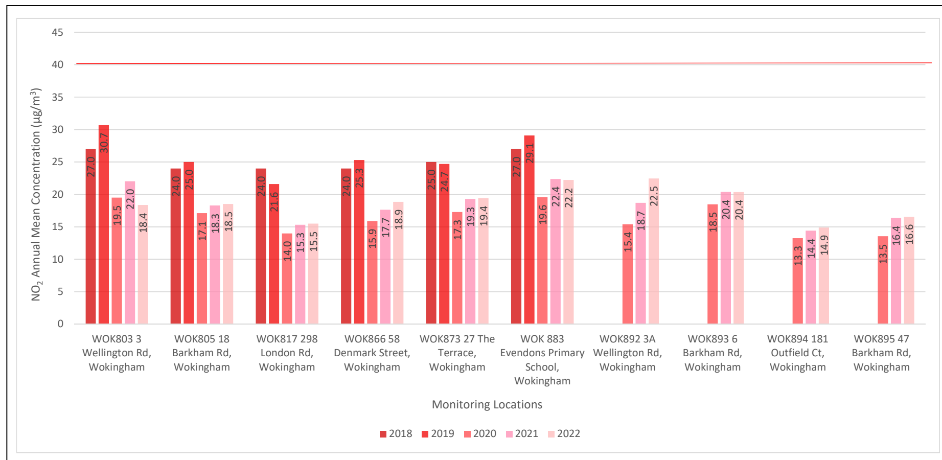
Figure A.4 – Trends in Annual Mean NO 2 Concentrations within Wokingham (outside the AQMAs) 2018-2022
