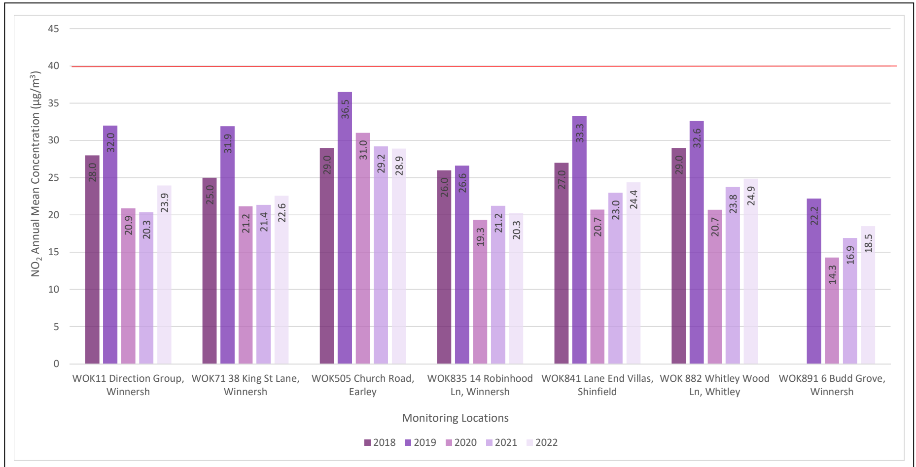
Figure A.5 – Trends in Annual Mean NO 2 Concentrations within Winnersh, Earley & Shinfield (outside AQMAs) 2018-2022
