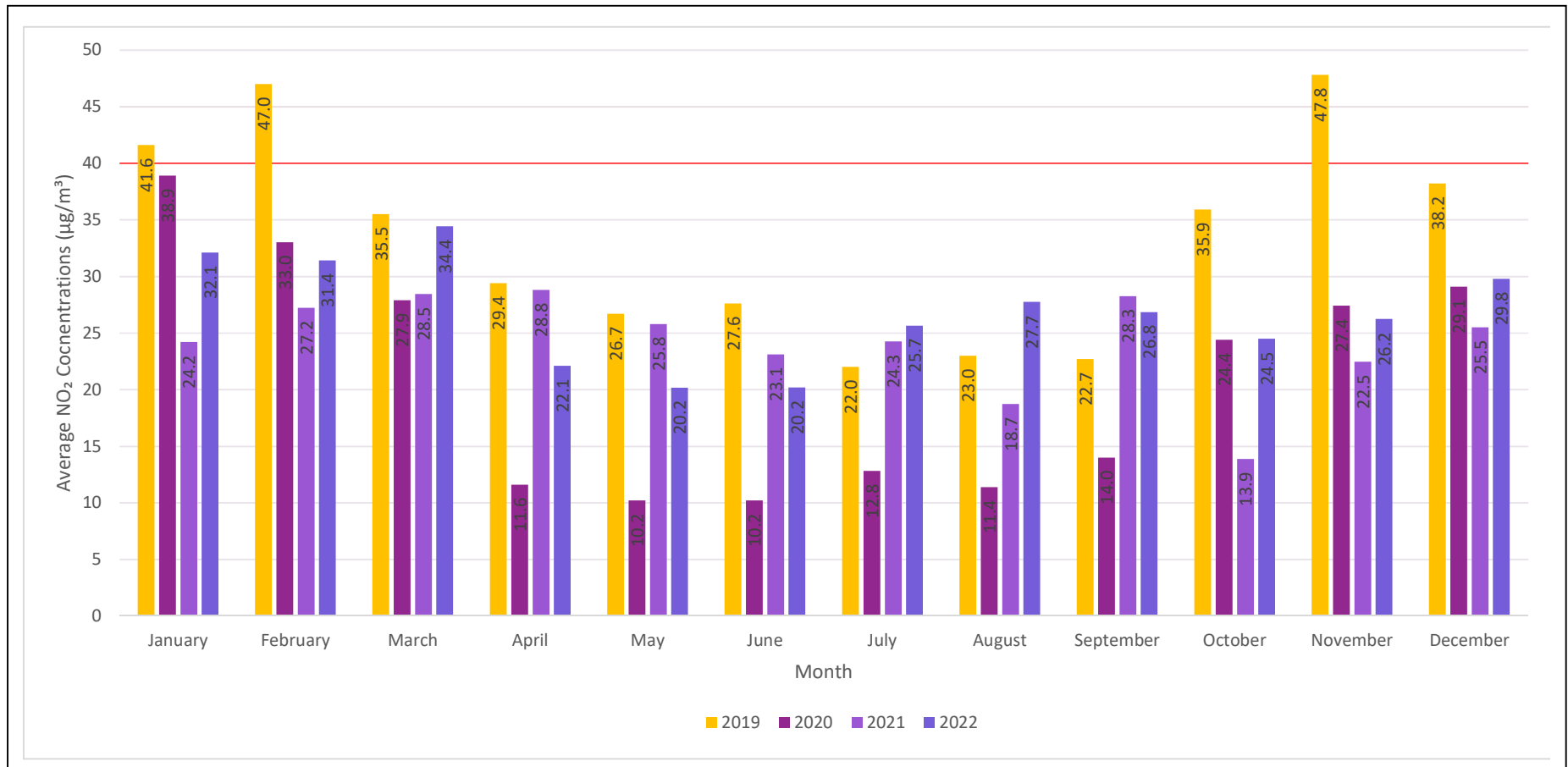
Figure A.7 – Trends in Monthly Average NO 2 Concentrations from Wokingham Continuous Monitor for 2019-2022
